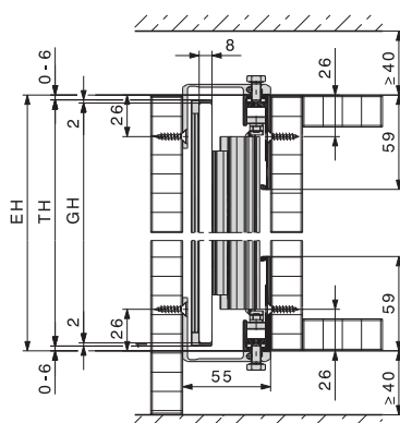
HAWA-Concepta 25/30 Connector: 55 mm
