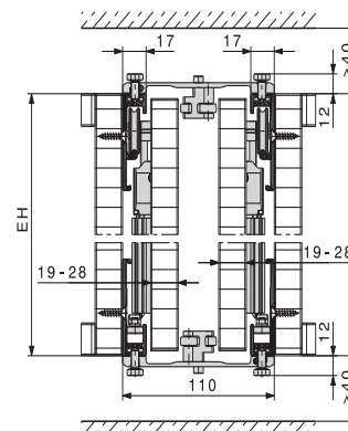
HAWA-Concepta 50 Connector: 110 mm
