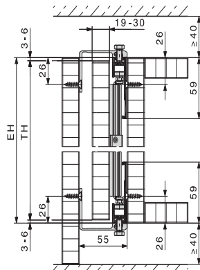
HAWA-Concepta 25/30 Connector: 55 mm
