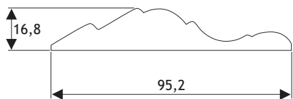
Type L1000-03 cache corniche
